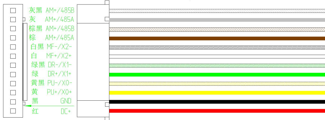
Figure 6.2 ISS28 series wiring diagram
