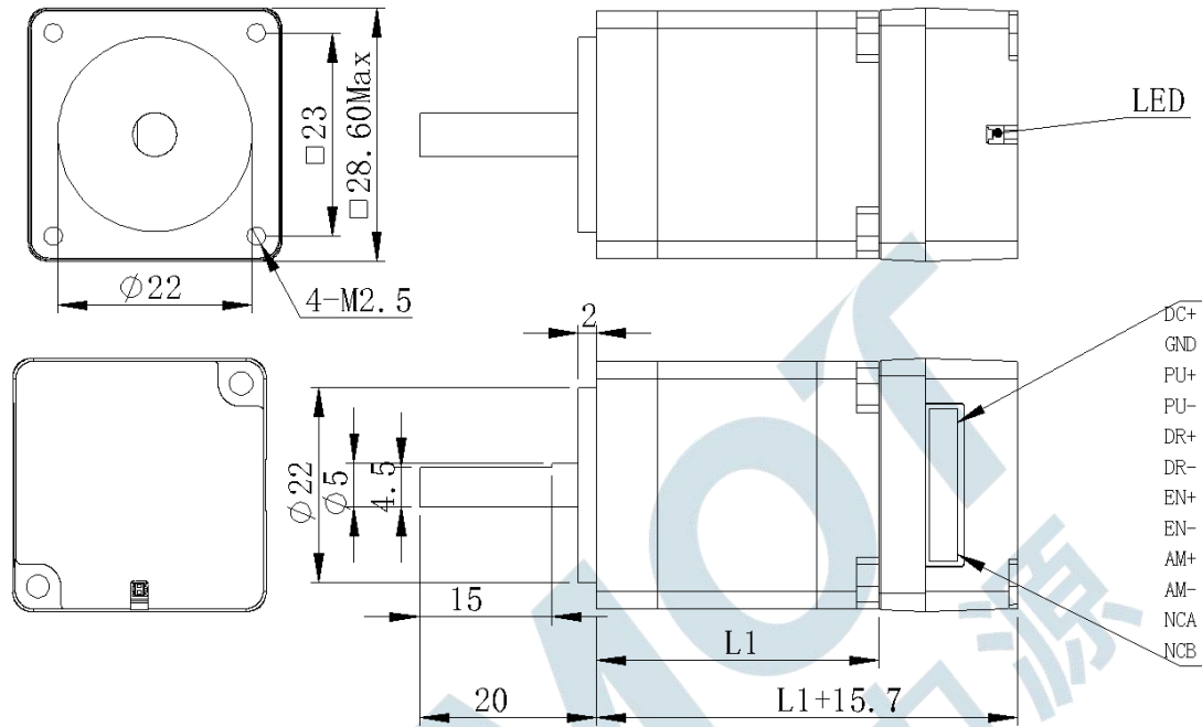
Figure 2.1 Installation dimensions (unit: mm)
