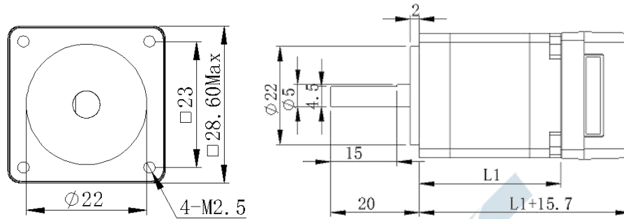
Figure 6.1 ISS28 Schematic diagram of the appearance of the series of integrated machines
